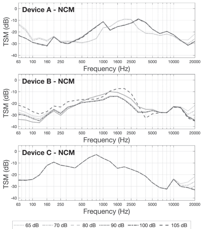
Figure 6. Total spectral modification of diffuse pink noise at presentation levels of 65–105 dB SPL for Noise cancellation modes for all devices.
