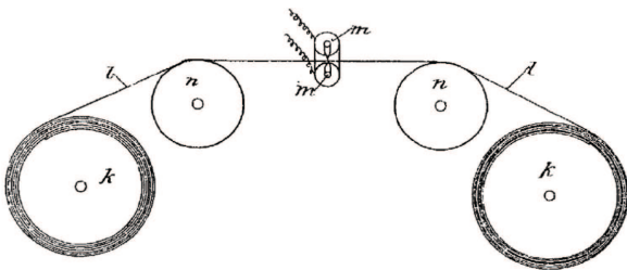
Figure 2. Alternative construction of the telegraphone. From the Danish patent No. 2653.
