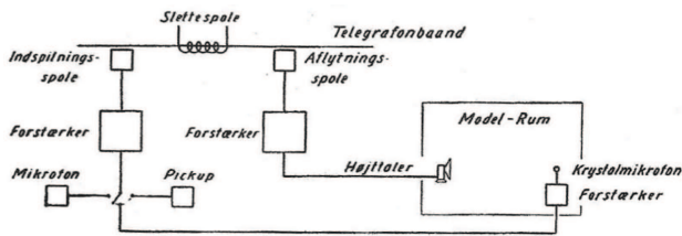
Figure 7. Diagram on the method for auralization in a scale model applied by V.L. Jordan. Adapted from [7, Fig. 49].
