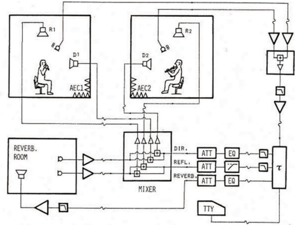
Figure 13. Setup for two musicians playing together involving two anechoic chambers, one reverberation room and a PDP 8 computer, Gade (1982).
