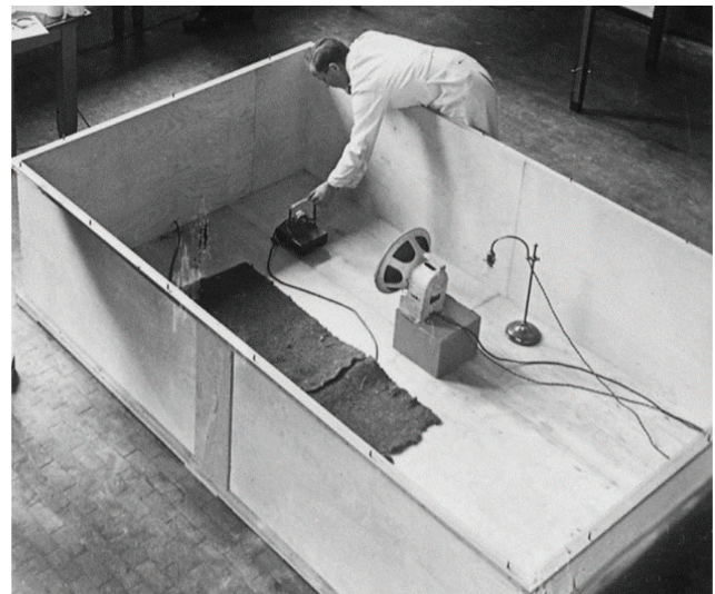
Figure 6. V.L. Jordan with the room acoustic scale model applied for auralization, around 1938.
