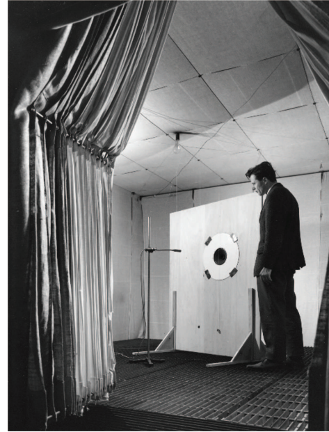
Figure 5. The anechoic chamber, built around 1935–40, 37 m 3 free volume. The person is Jørgen Kristensen.
