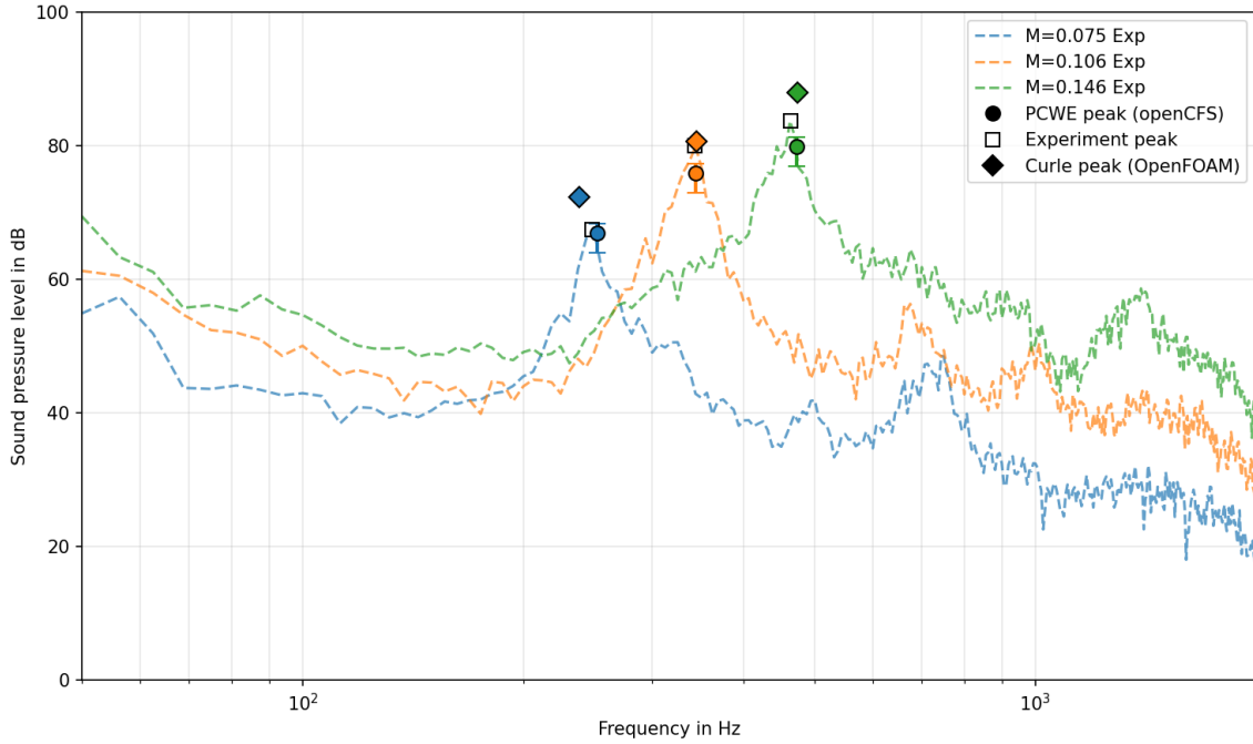
Figure 9: Sound pressure level spectra (ref 20 \mu\text{Pa} ) obtained for the 20 mm diameter cylinder models in comparison to the aeroacoustic simulation using the PCWE and Curle's analogy.
