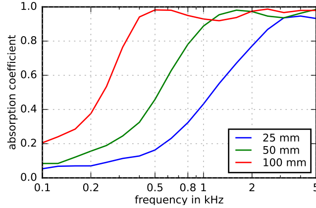
Figure 2: Absorption coefficients of the material with which the wind tunnel test section is lined, taken from the data sheet for different standard thicknesses [11].
