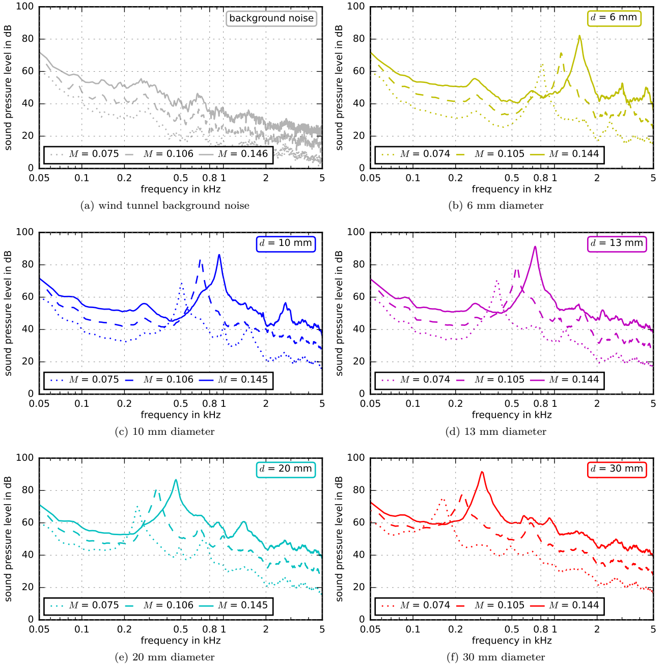
Figure 4: Sound pressure level spectra (re 20 \mu\text{Pa} ) obtained for the different cylinder models and the wind tunnel background noise at three flow velocities U_0 .
