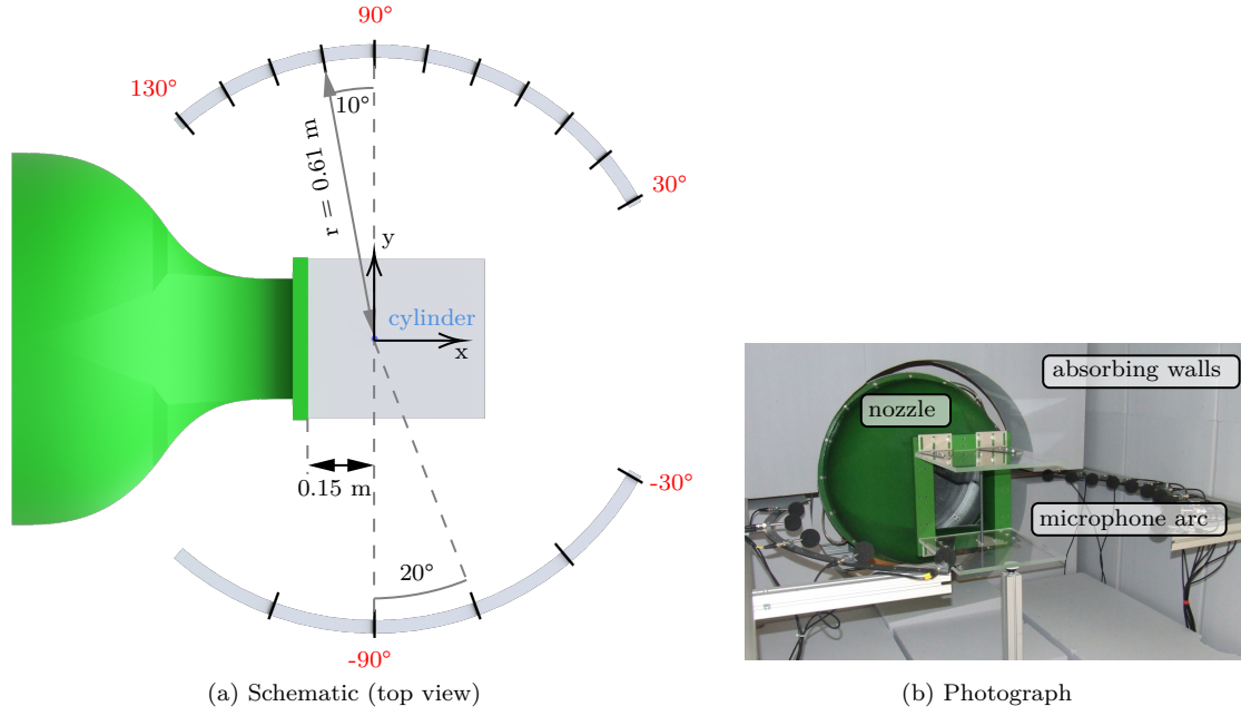
Figure 1: Experimental setup in the aeroacoustic wind tunnel.
