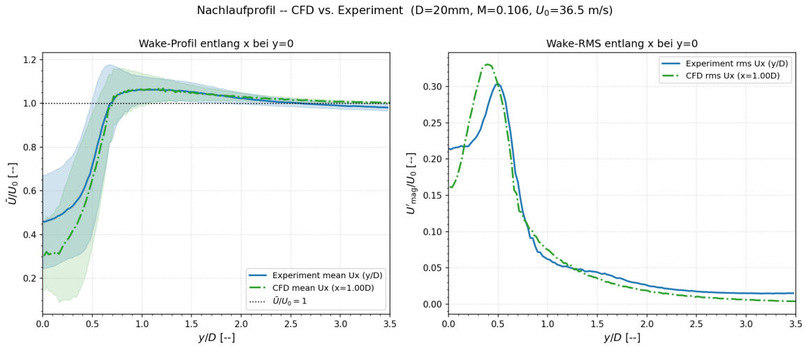
Figure 8: Validation of the flow (half-)profiles of the streamwise velocity component measured and simulated in the wake of the cylinders at a downstream distance of 1d from the cylinder axis at a nominal flow speed U_0 of 36.5 m/s ( M = 0.106 ).
